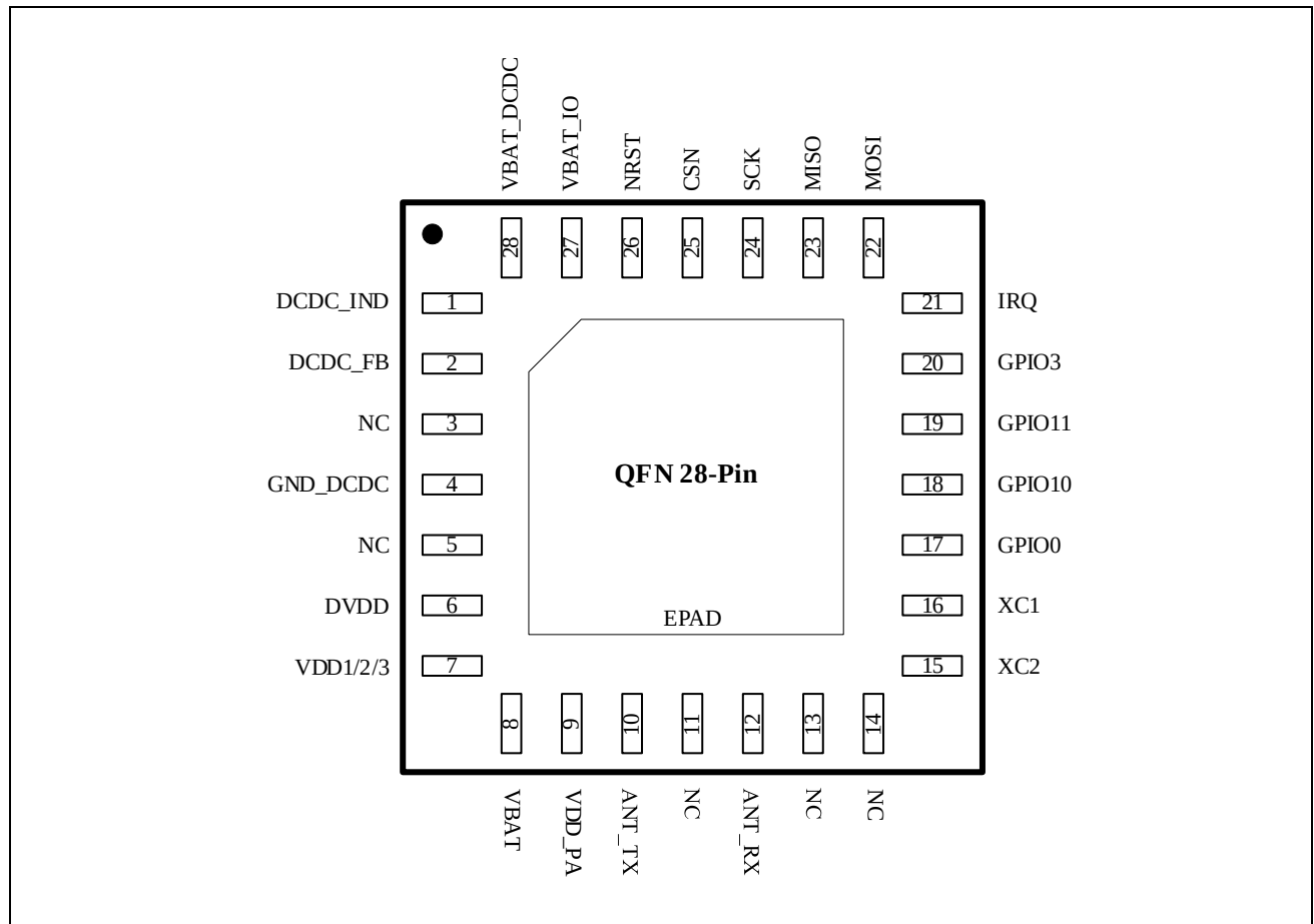
Figure 4-1 Pin diagram
